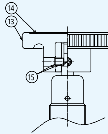
Construction of handle part (Nominal Size 1/4)
